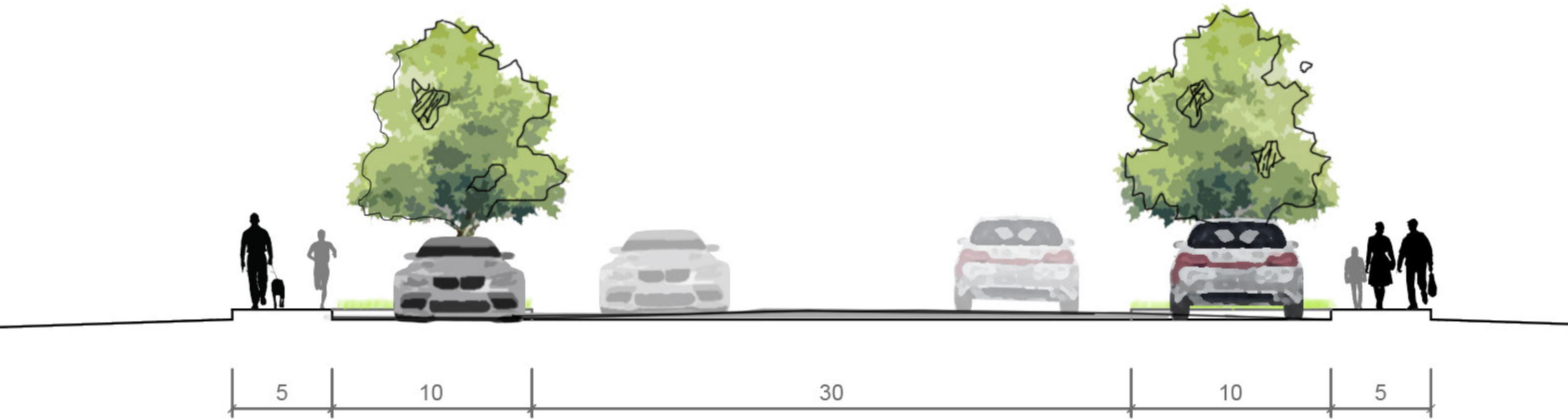
SECTION B-B'
